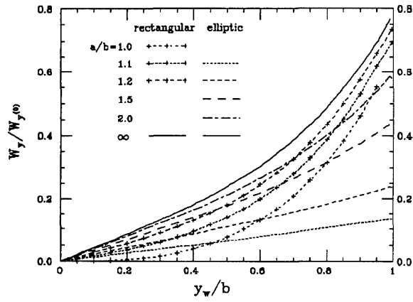
Figure 2: Vertical asymptotic wake vs. the location of the witness particle for rectangular and elliptic pipes of various aspect ratio with fixed vertical aperture.
