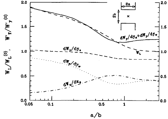
Figure 4: Asymptotic wake for finite width parallel collimator for r_w = r_s = 0 . (width 2a , gap height 2b ) Normalized by the corresponding wake for a round pipe with radius b .
